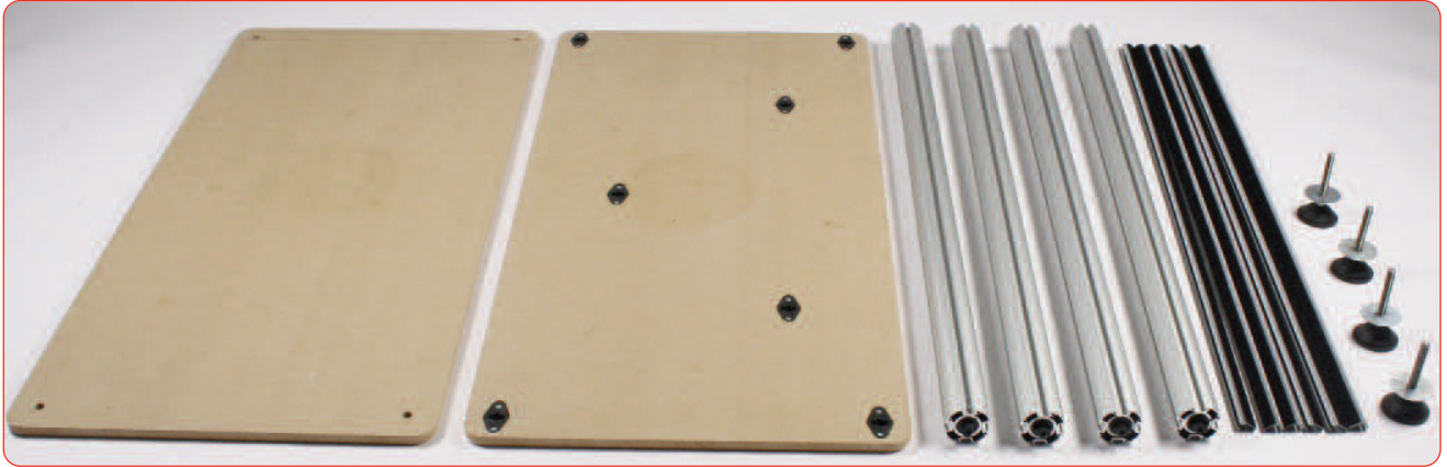
Kit Includes: 1x table top, 1x base, 4x linear 50mm round post, 4x adjustable fit, 6x wing extrusion Kit based on LK029-001
