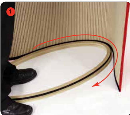
1 Place the base (A) on the floor and begin to secure the wrap (C) around the hook fastener strip.
